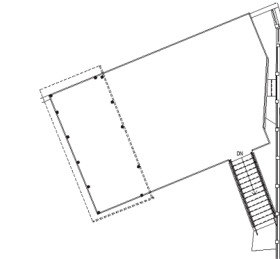
2 LEVEL 2- FLOOR PLAN 1/8" = 1'-0"
