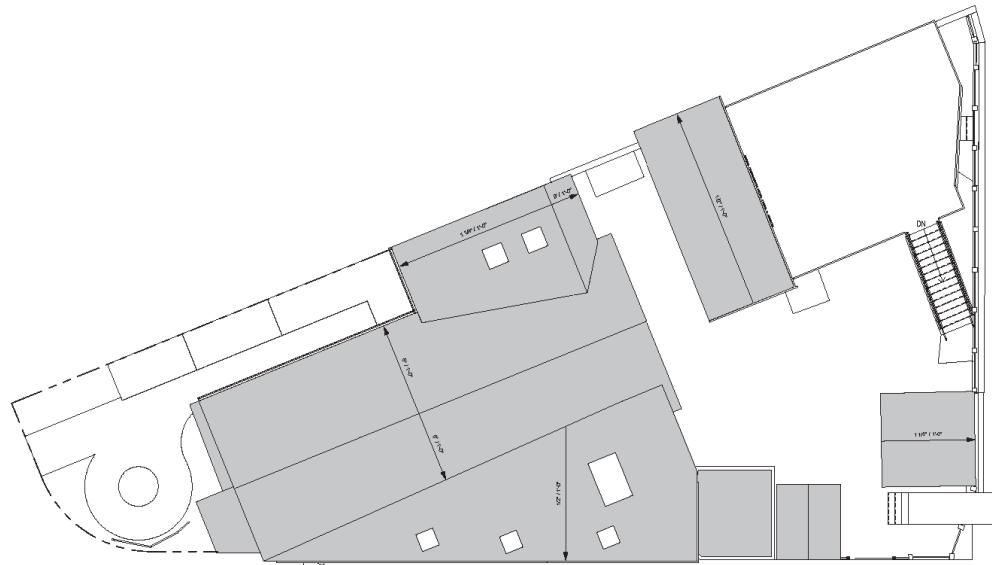
1 LEVEL 1- FLOOR PLAN 1/8" = 1'-0"
