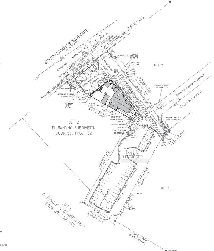
4 SURVEY OVERLAY 1" = 50'-0"
